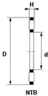
THRUST NEEDLE&RETAINER ASSEMBLY NTB
